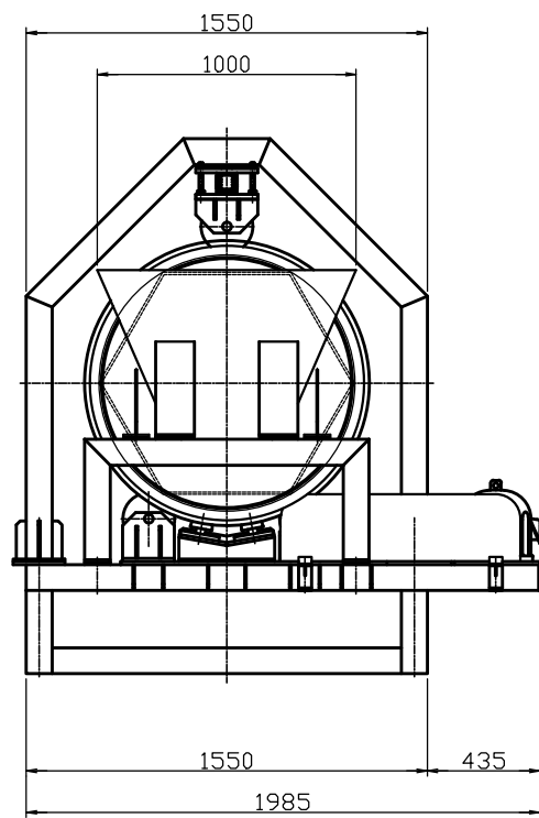
B~矢視
